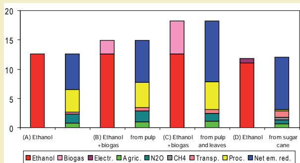
Figure 2. Gross and net GHG emission reduction (ton CO 2 -eq./ha) for sugar beet ethanol (A, B, C) and biogas (B, C) as well as sugar cane (D) production. See text for explanation.
