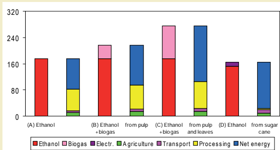
Figure 1. Gross and net energy production (GJ/ha) from sugar beet ethanol (A, B, C) and biogas (B, C) as well as sugar cane (D) production. See text for explanation.
